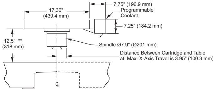
Detail C
