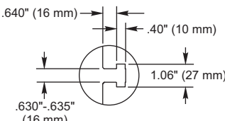
Detail B (5X)
