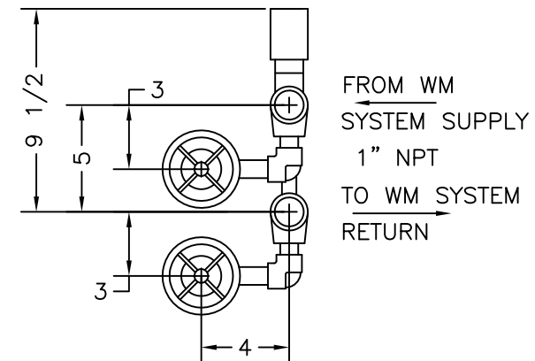
END VIEW
